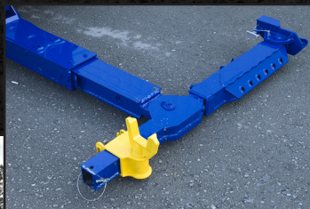
The 2465 comes standard with a low-profile crossbar with removable ends, one set of lift forks, fork holders and a 6,000-lb. pivoting L-Arm System.
